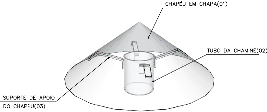
PERSPECTIVA 3D
